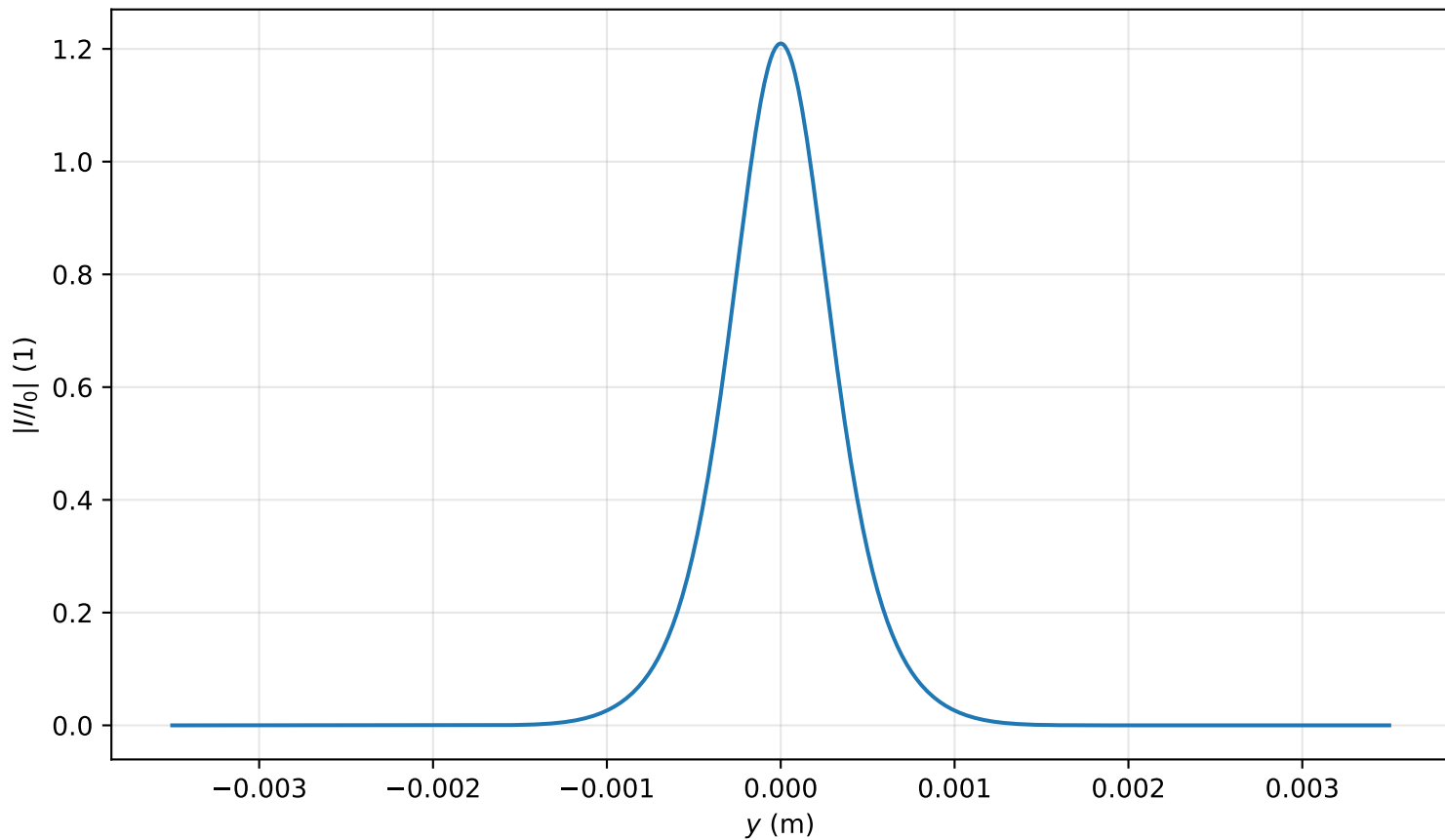
Intensity profile I(x=0, y, z=1.115)/I_0 , P_{in}=0.7P_{cr} , artificial time
